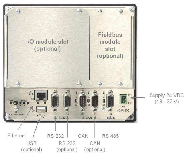
Fig. 2: Connections KS 108 PLC
