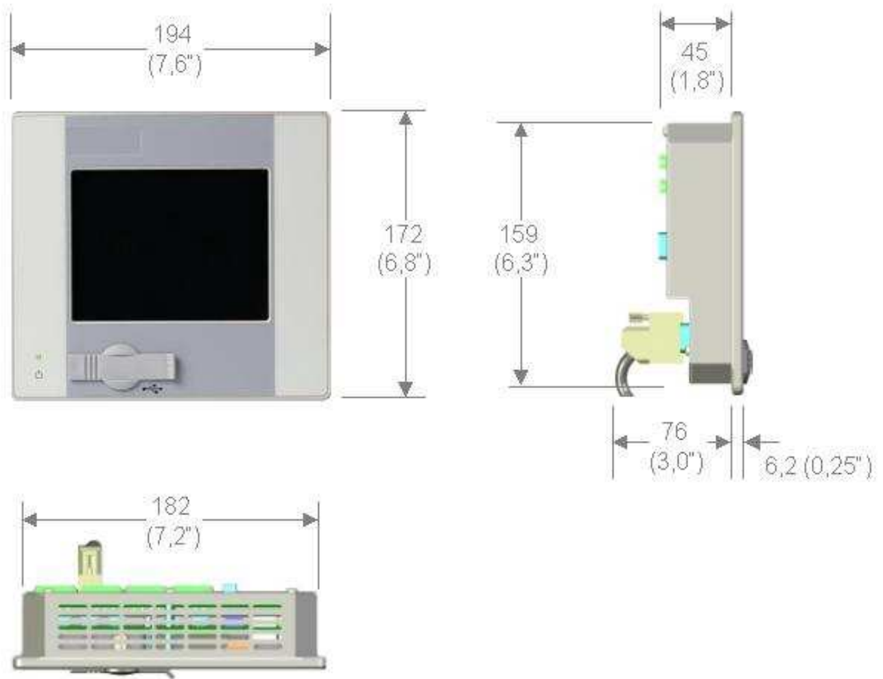
Fig. 1: Overall dimensions KS 108 PLC
